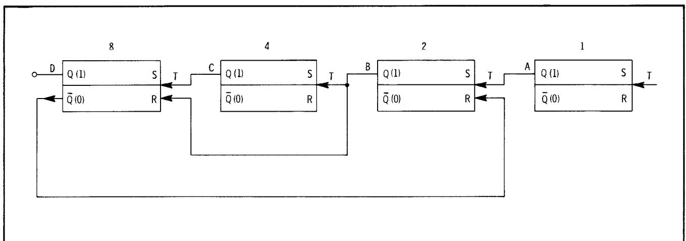
Figure 8-12. 8421 BCD Decade Counter
