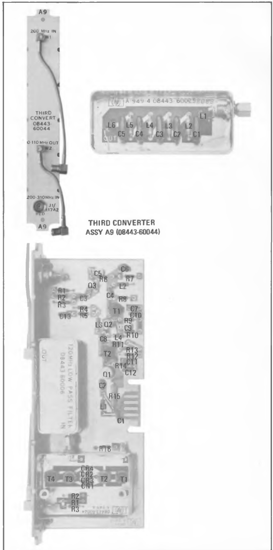
Figure 8-25. A9, Third Converter Assembly
