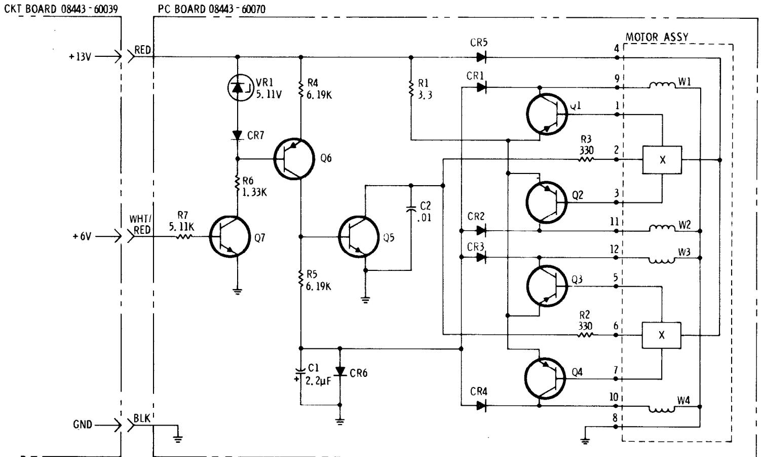
Motor/Driver Circuit Diagram
