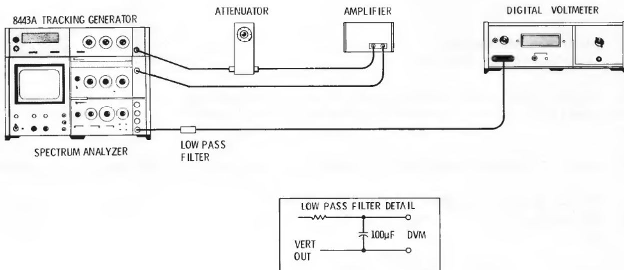
Figure 4-2. Amplitude Range Test Setup
