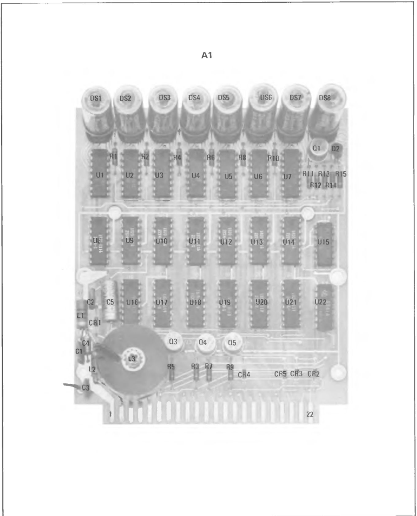
Figure 8-38. A1, Low Frequency Counter Assembly, Components
