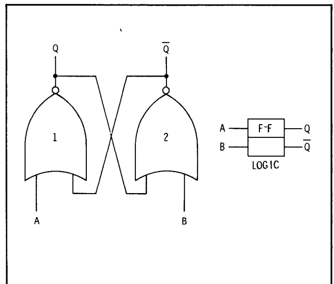
Figure 8-5. Basic NOR Gate Flip-Flop
