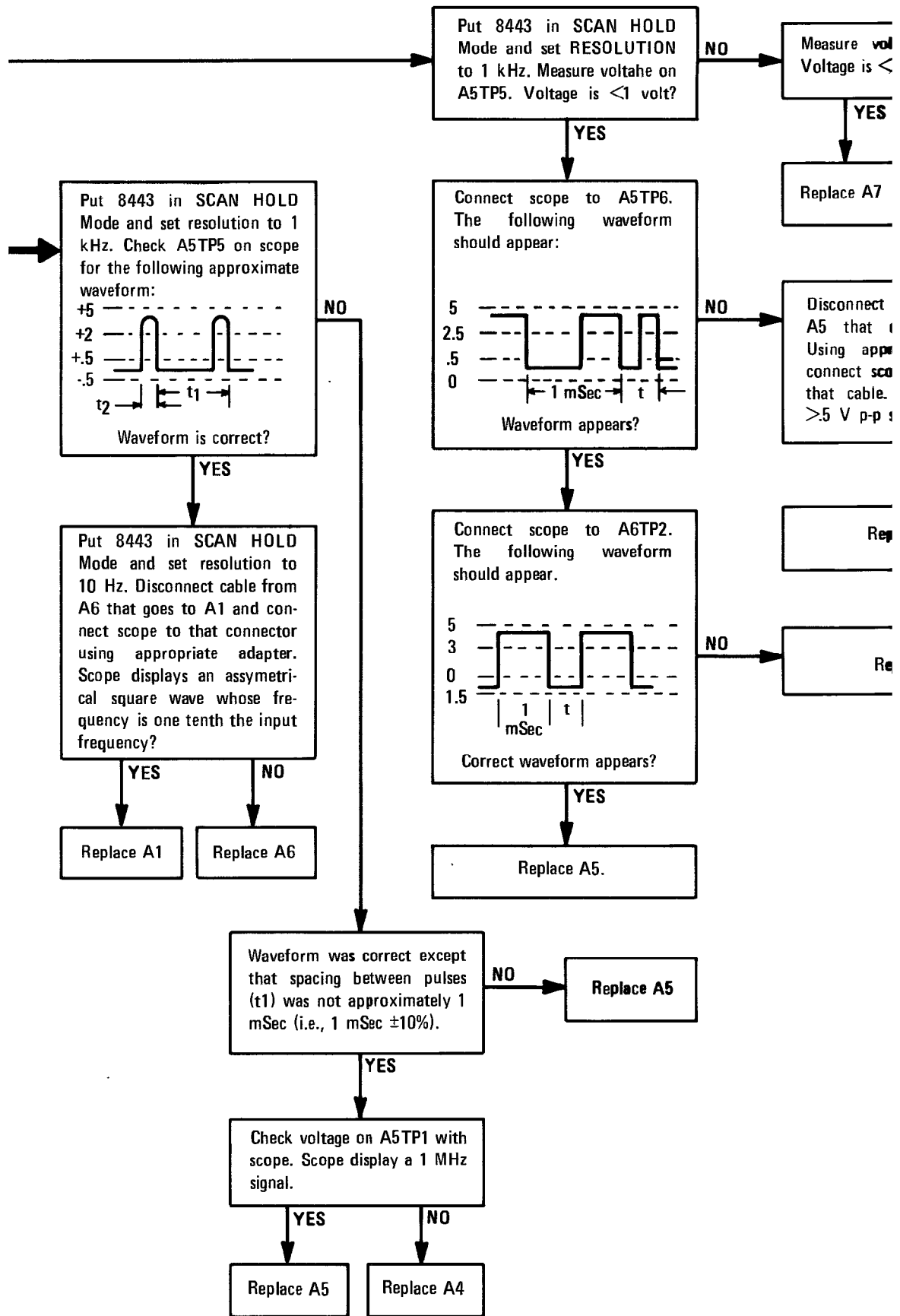
ROUBLESHOOTING TREE
