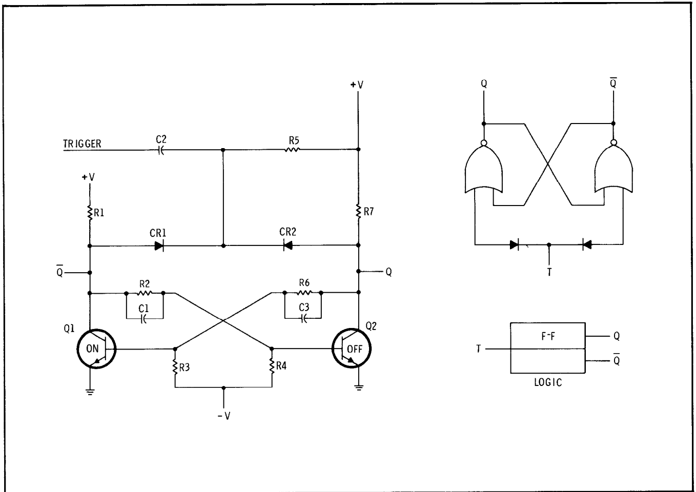
Figure 8-6. Triggered Flip-Flop
