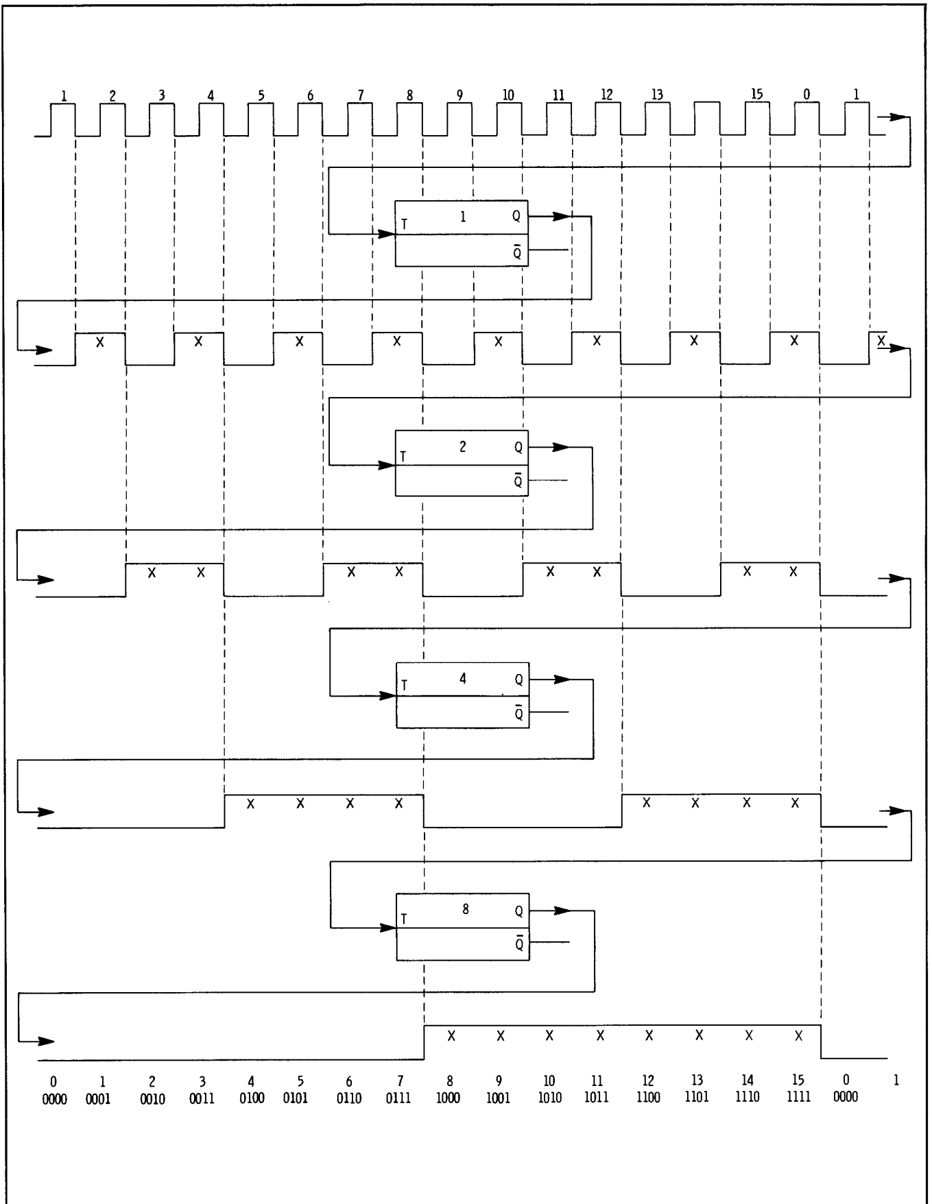
Figure 8-11. 16 Counter Binary Counter Chain
