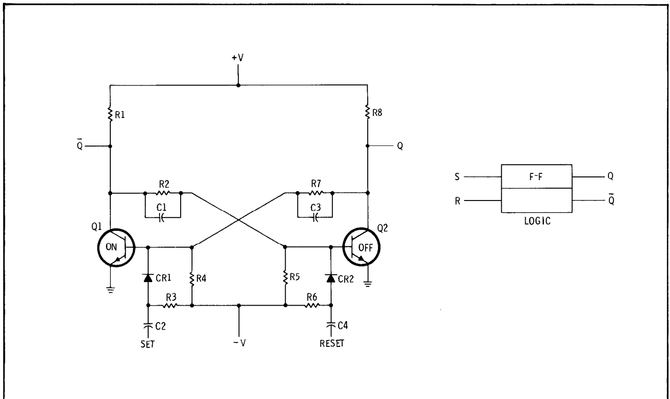
Figure 8-7. RS Flip-Flop
