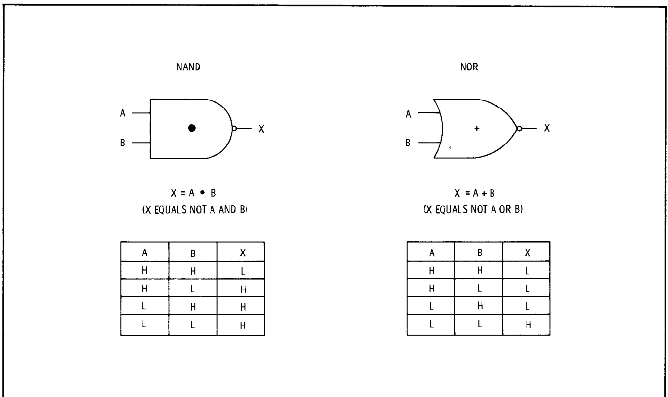
Figure 8-3. Basic NAND and NOR Gates
