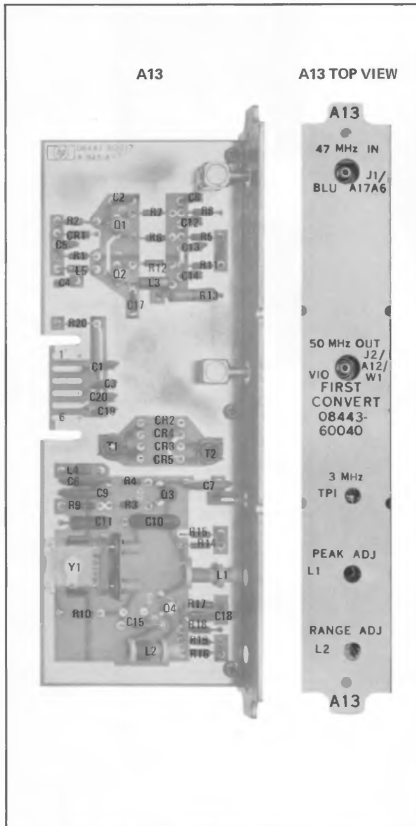
Figure 8-21. A13, First Converter, Cover and Components
