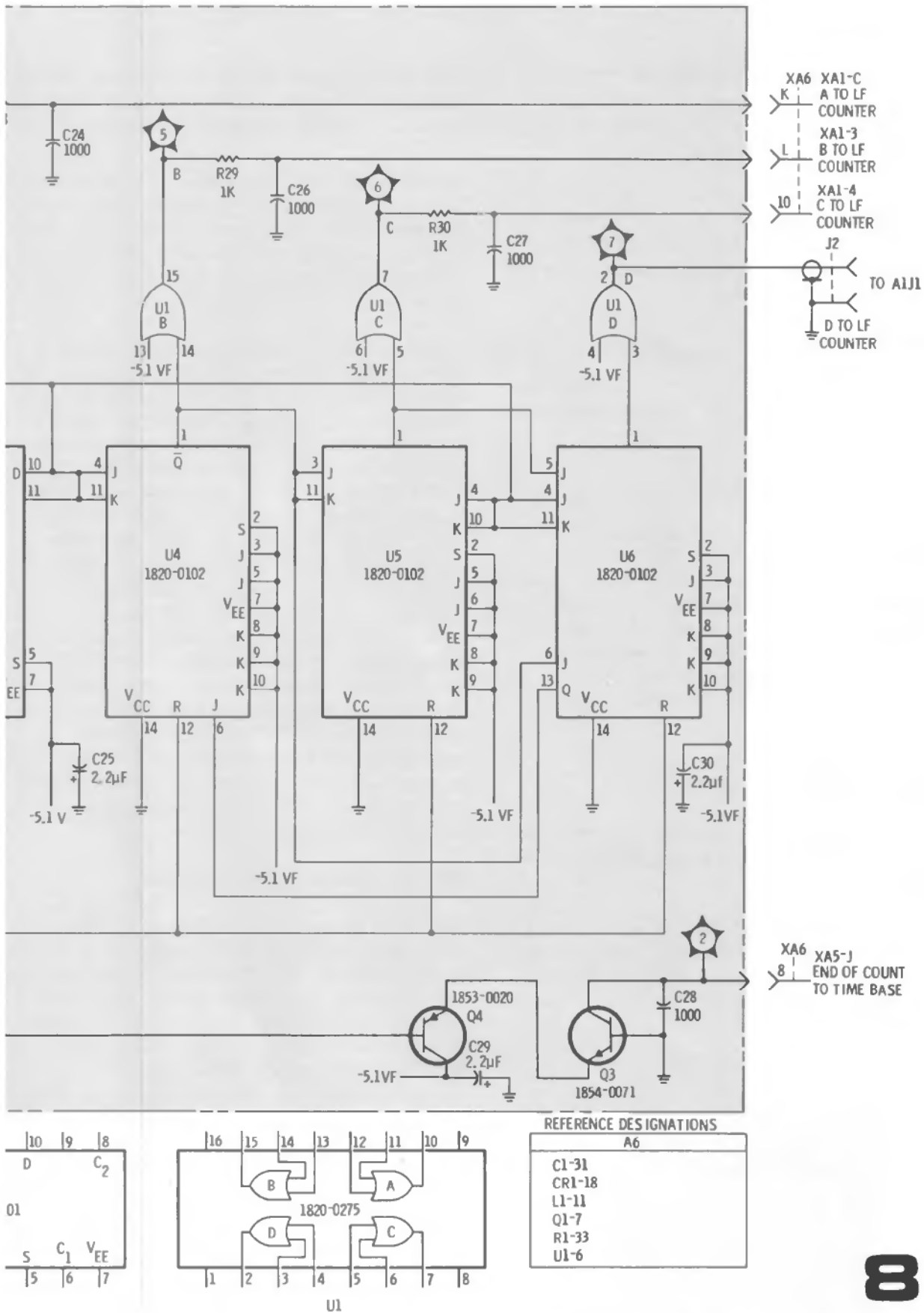
Figure 8-37. High Frequency Decade Assembly, Schematic Diagram
