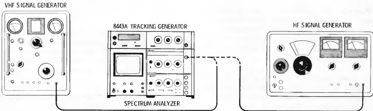
Figure 4-1. Frequency Range Test
