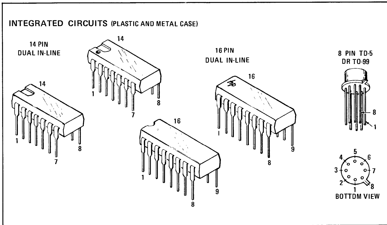
Figure 8-16. Integrated Circuit Packaging
