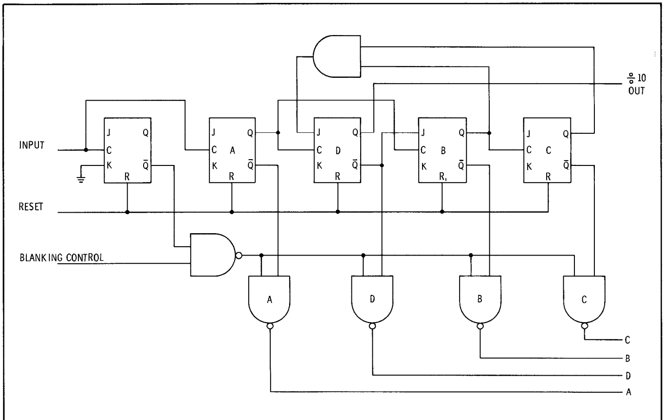
Figure 8-13. Blanking Decade Counter
