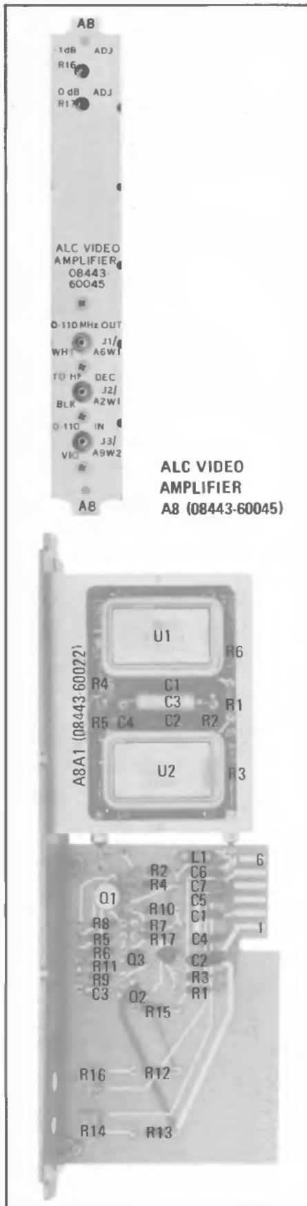
Figure 8-24. A8, ALC Video Amplifier
