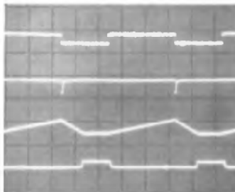
Waveform SS6-4
