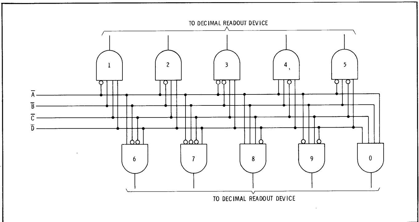
Figure 8-15. Decoder
