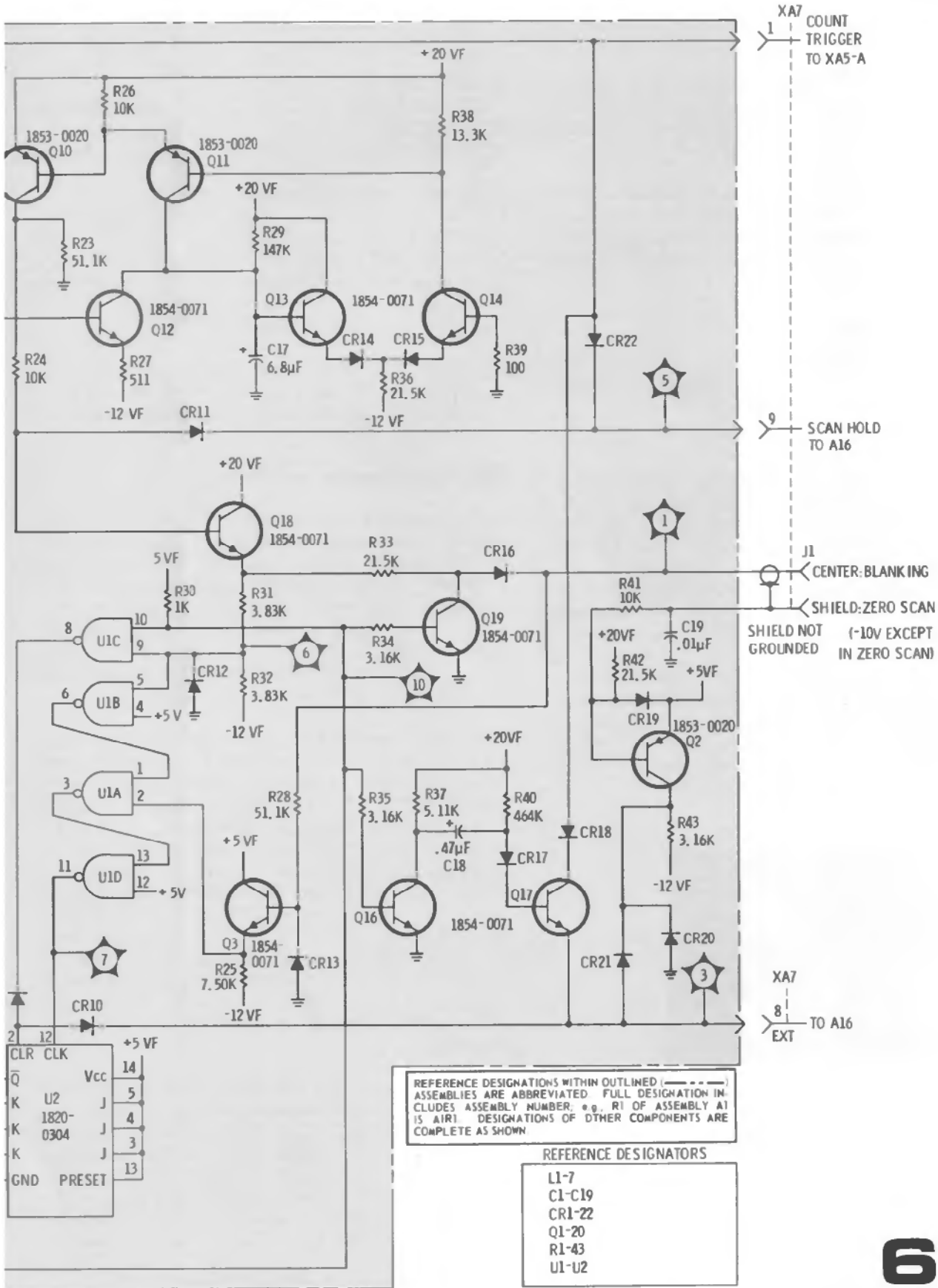
Figure 8-33. Marker Control Circuit, Schematic Diagram
