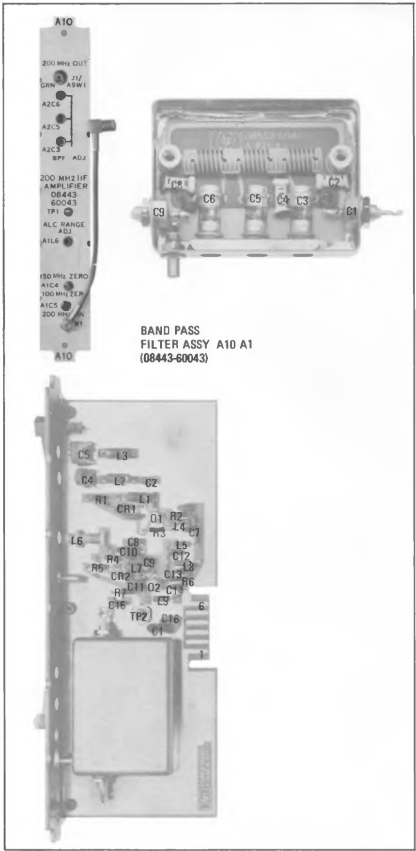
Figure 8-26. A10, Bandpass Filter Assembly
