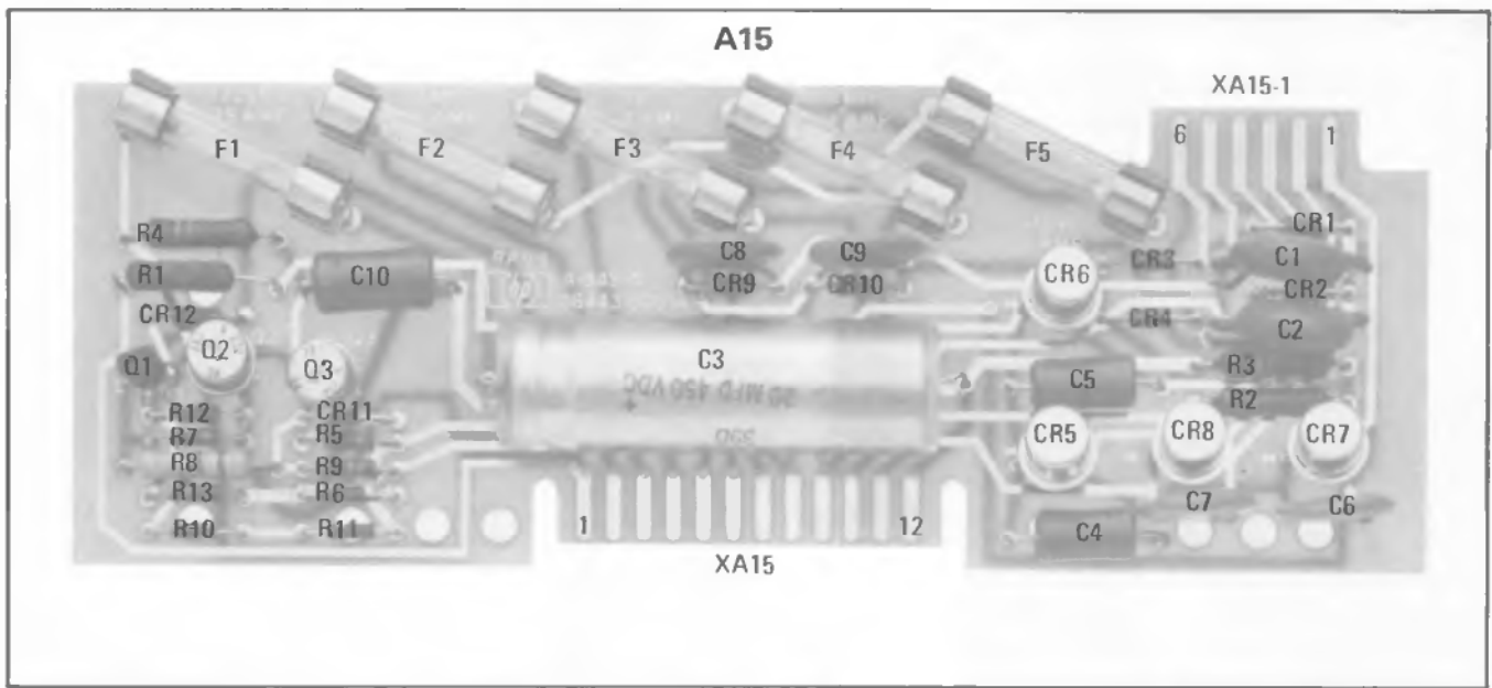
Figure 8-29. A15, Rectifier Assembly, Components
