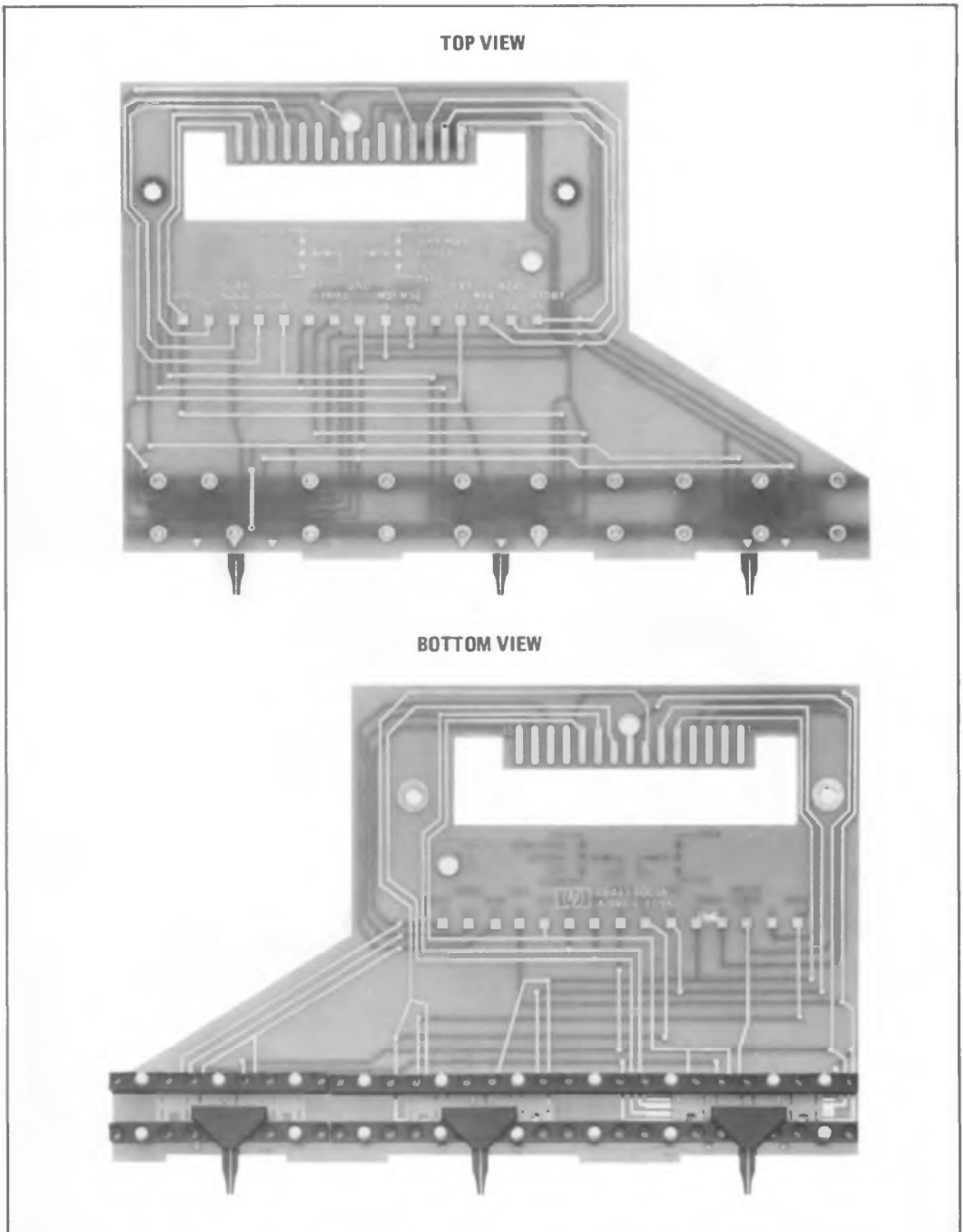
Figure 8-41. A16, Switch Assembly
