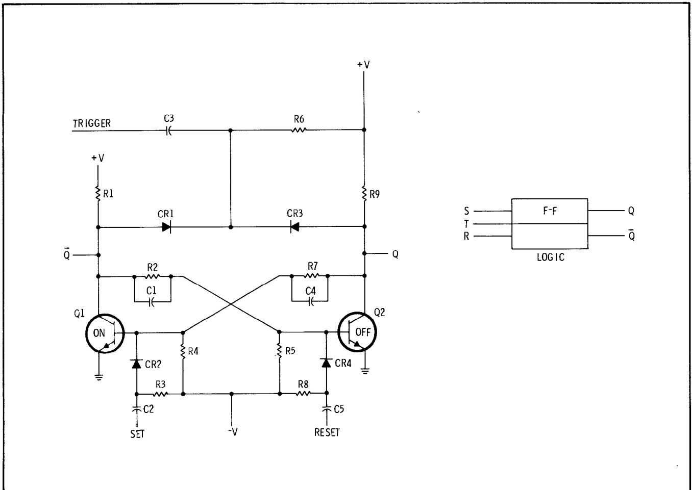
Figure 8-8. RST Flip-Flop
