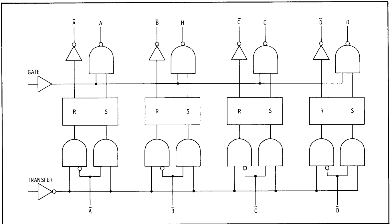
Figure 8-14. Buffer/Store
