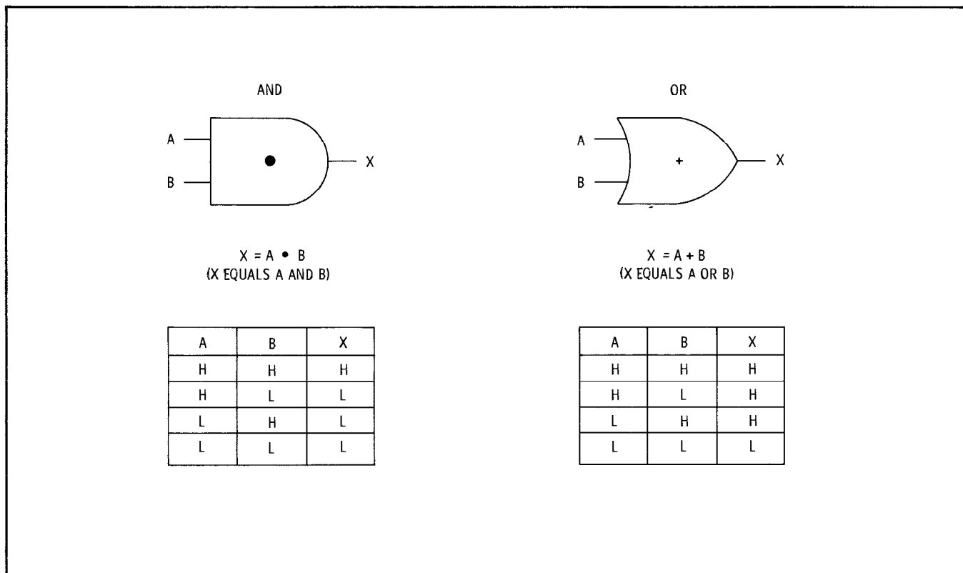
Figure 8-2. Basic AND and OR Gates
