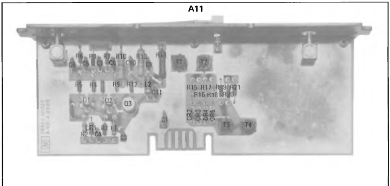
Figure 8-20. A11 Second Converter, Cover and Components
