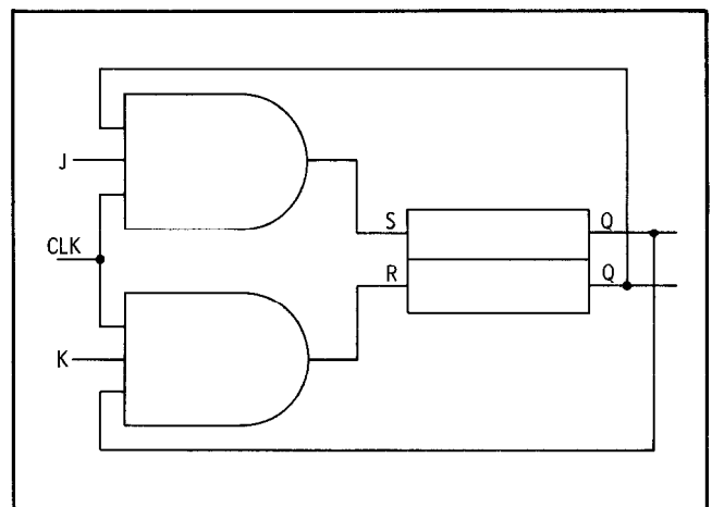
Figure 8-9. Clocked JK Flip-Flop
